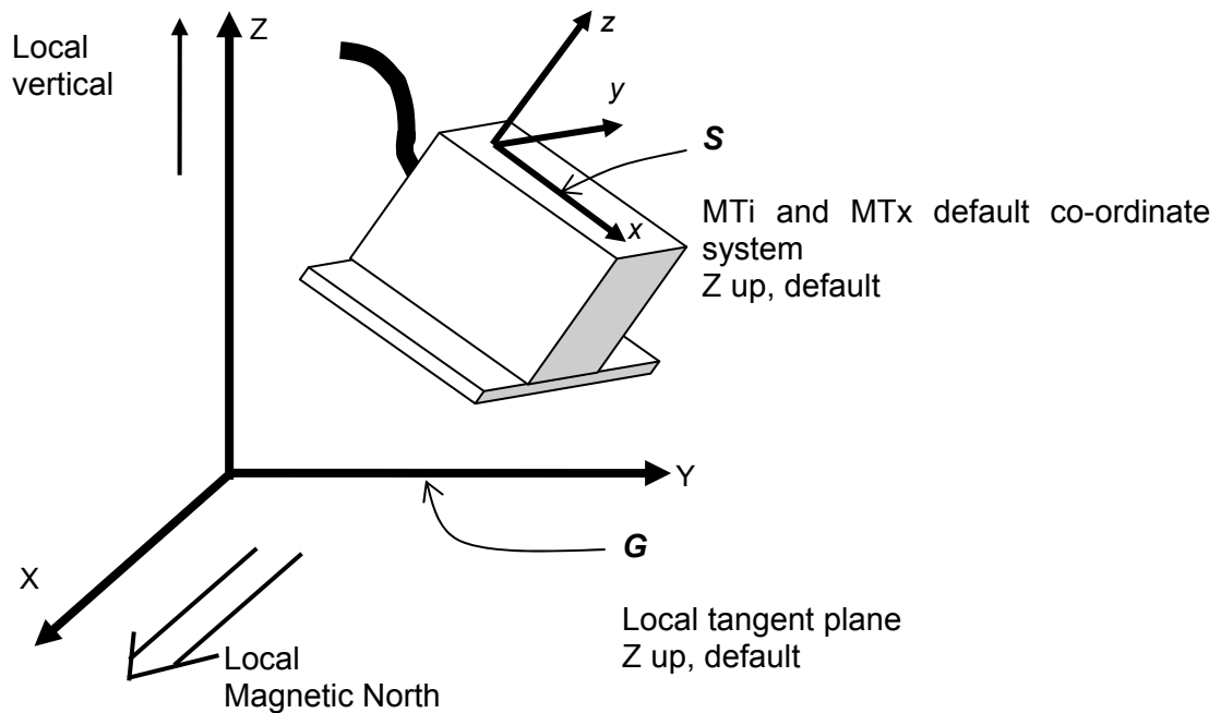
Figure 3: MT in the earth-fixed co-ordinate system
